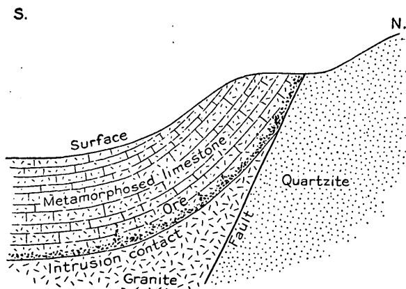
FIGURE 67.—Diagrammatic section showing probable general relations of the ore to the enclosing rocks at Mineral Hill, Pima district, Ariz.
